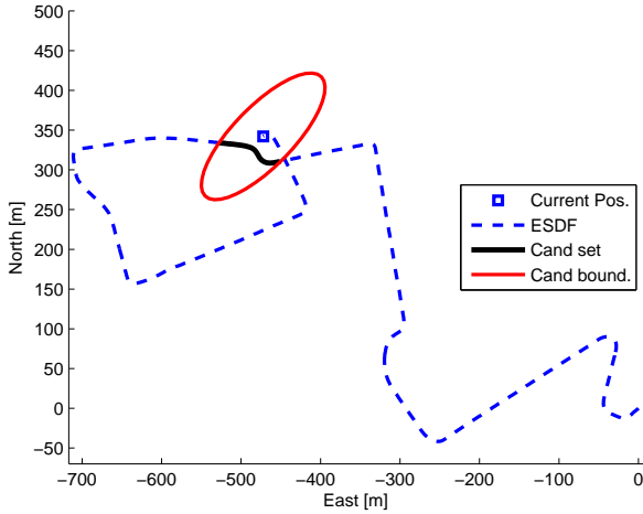
Figure 2: Loop closure candidates, indicated by the ellipse. The 50 last augmented states are excluded.
