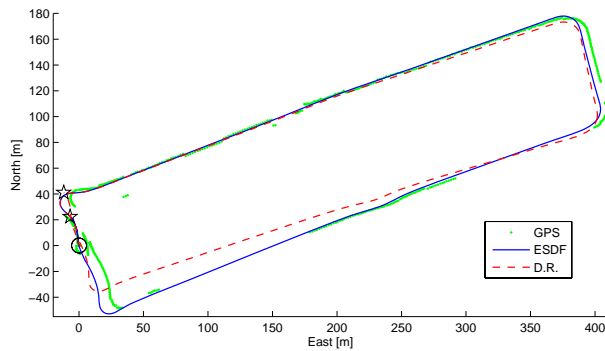
(c) Estimated trajectory compared to dead reckoning (D.R.) and GPS.
