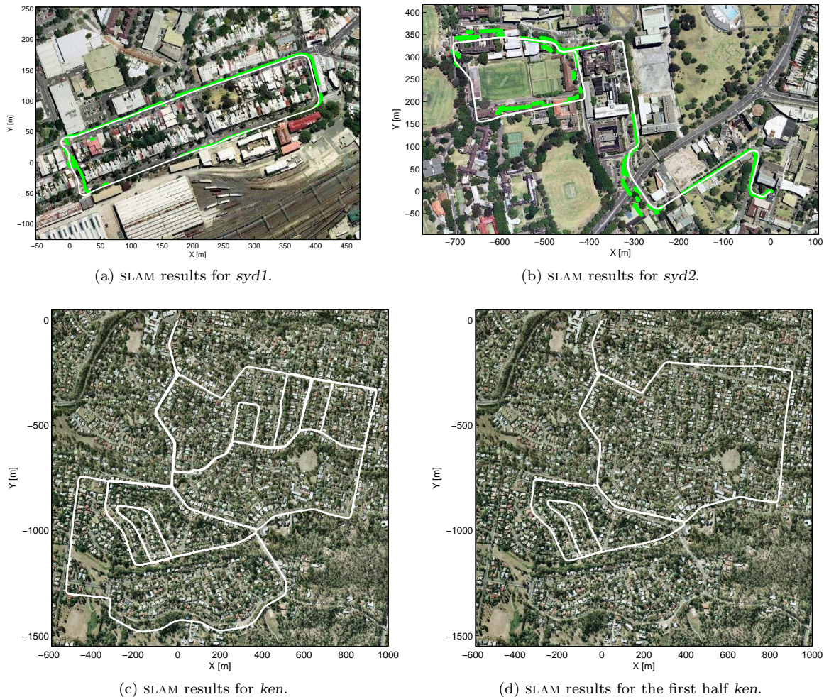
Figure 3: Estimated SLAM trajectories (white) overlaid on Google maps images, and compared to GPS (green) when available. Note that the GPS signal becomes increasingly unreliable under trees and tall buildings. The SLAM trajectories were used to find point cloud pairs for training and evaluation of the classifier.
