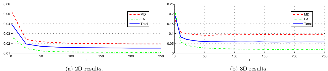
Figure 4: Error rates during AdaBoost training plotted against the number of training rounds T . For both 2D and 3D data the validation error levels stop decreasing after about 50 training rounds, hence T = 50 is an appropriate choice for the subsequent experiments.
