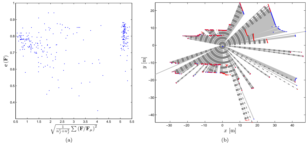
Figure 9: Results from experiment with dynamic objects. (a): Comparison of classifier likelihood and feature difference, computed as (24). Despite large feature differences, reasonable classification likelihood can still be achieved in many cases. (b): Example of point cloud pair, where the appearance of the scene is changed by dynamic objects. The first point cloud is shown as blue dots, with the measurement rays shown in light gray. The other point cloud is shown as red dots, with the measurement rays shown in dash-dotted dark gray. The feature difference is 5.31, the classification likelihood, 0.53 is quite low. Note that range measurements at maximum range are not plotted for increased clarity.
