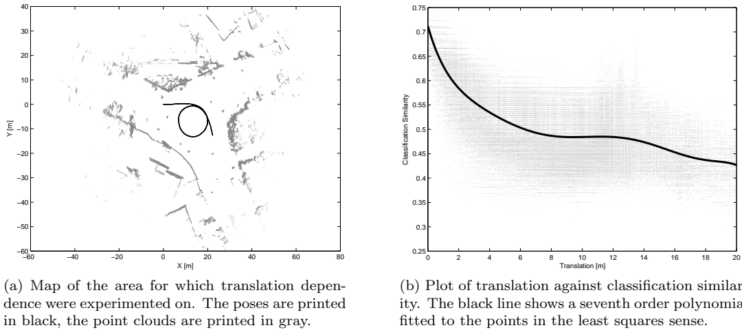
Figure 7: Classifier dependence to translation.
