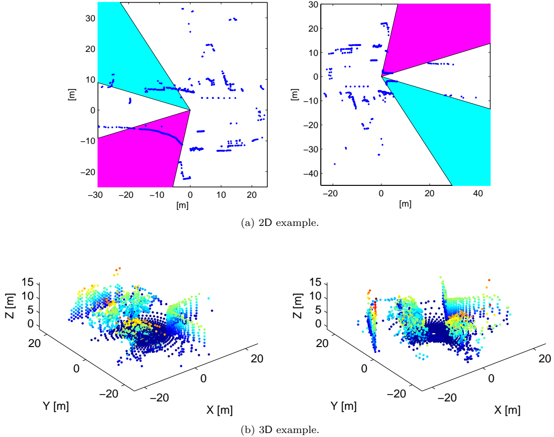
Figure 1: Examples of the loop closure detection problem. In (a) two planar point clouds from the same location are shown. Parts of the scene are occluded by vehicles parked along the side of the road in the right point cloud, these parts are highlighted in colour. In (b) two 3D point clouds are shown, colour is used to accentuate the height. These point clouds are from the same location, which can be identified by the building corner and the wall opposite the corner.
