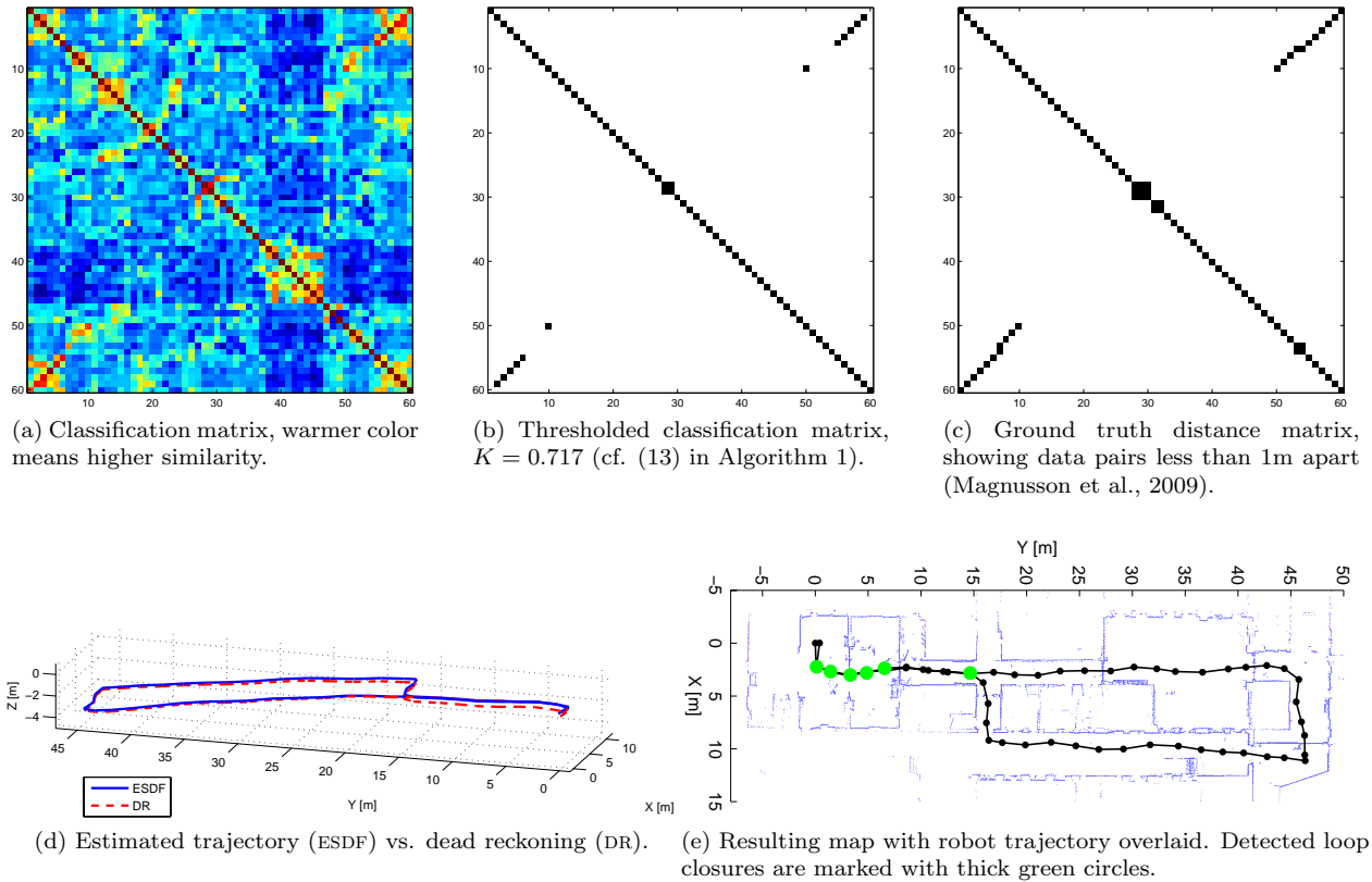
Figure 12: Results from SLAM experiment on AASS data.
