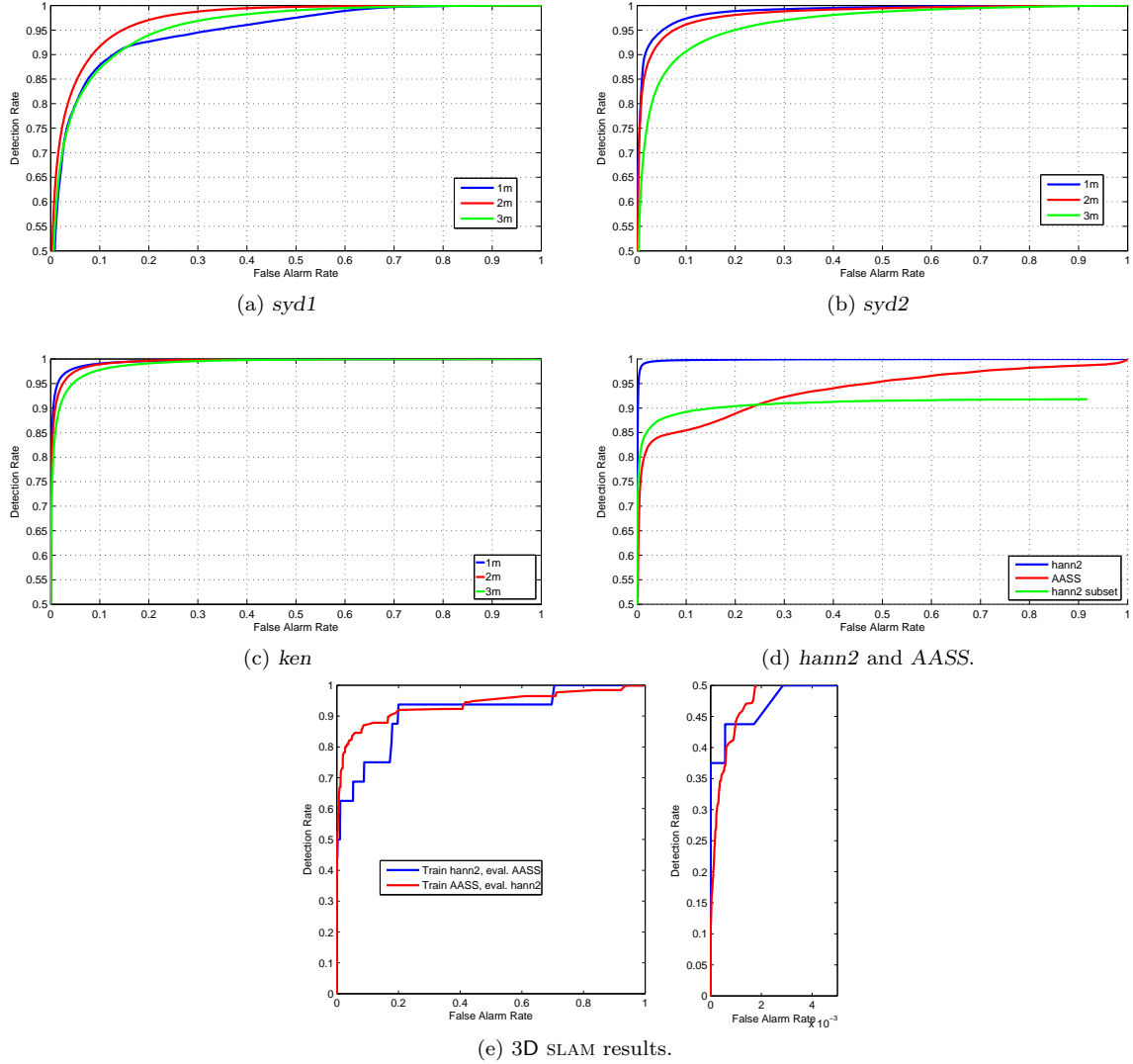
Figure 5: Receiver operating characteristic (ROC) curves. For each level of false alarm, the higher the detection is, the better the classifier is.
