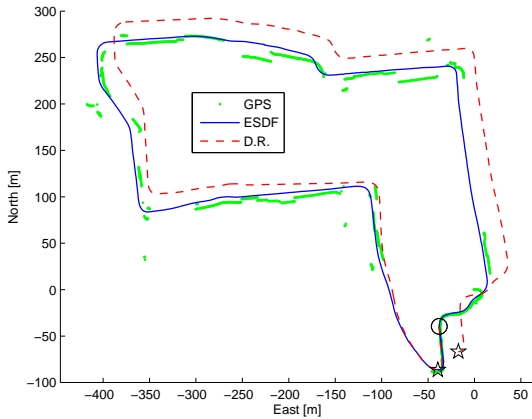
(a) Estimated trajectory compared to dead reckoning (D.R.) and GPS.
