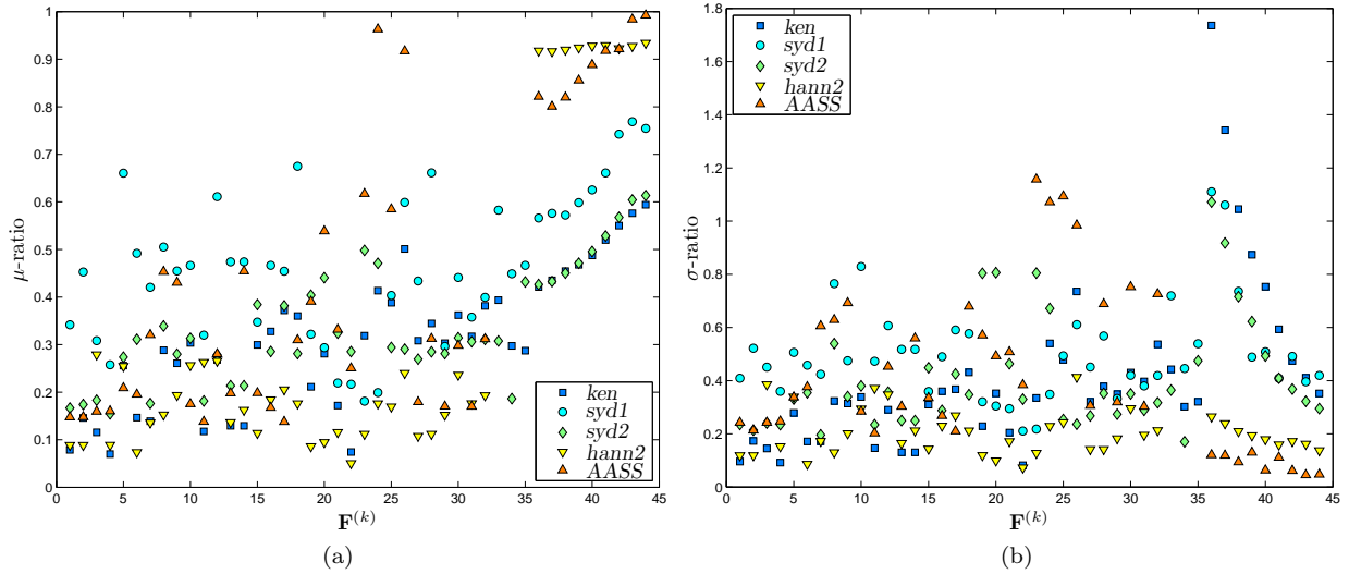
Figure 10: Results from repetitive structures experiment. The plots show the ratio for the positive and negative data pairs of mean, in (a), and standard deviation, in (b), of the extracted features. Ratios close to, or larger than one, suggest a high degree of repetitive structures.
