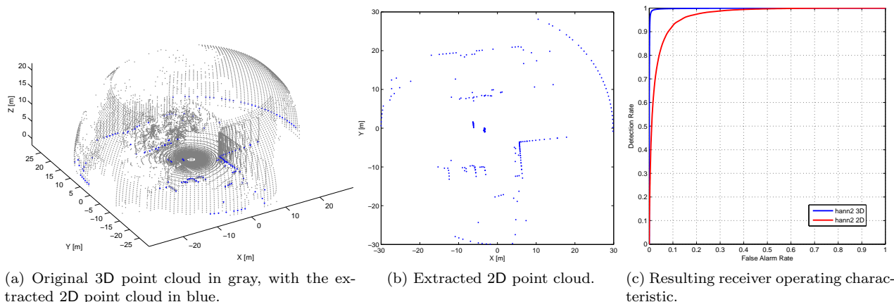
Figure 6: Illustration of the extraction of 2D point clouds from 3D point clouds.
