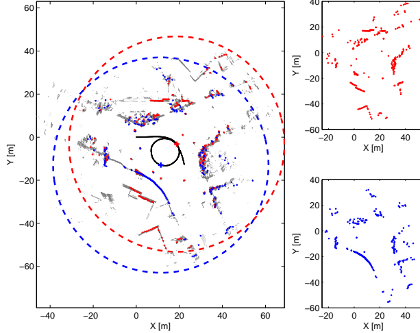
Figure 8: Illustration of the translation problem, for 2D data in outdoor environments. The plot on the left shows a trajectory, black line, along which 1000 point clouds were acquired, the constructed area map is shown in gray. Two poses are marked by crosses in blue and red, respectively, and the corresponding sensor surveillance boundary is shown by the dashed circles. Despite the fact that the relative pose translation, 12m, is well below the sensor’s maximum range, 50m, the point clouds corresponding to the poses are significantly different.
