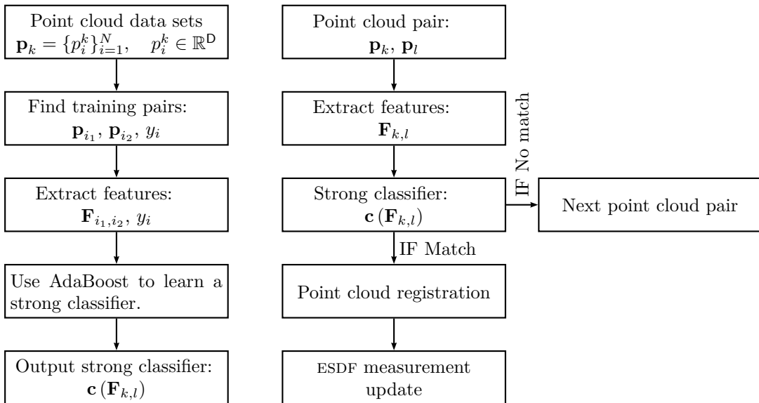
Figure 2: Algorithm overview. Left diagram, learning phase. Right diagram, classification phase. In the learning phase, one or more point cloud data sets are used to learn a strong classifier. The learning phase is run first in our algorithm. In the classification phase the strong classifier is used to detect loop closure in SLAM experiments. In our SLAM implementation, the classification phase is run each time a new pose has been added to the state vector.
